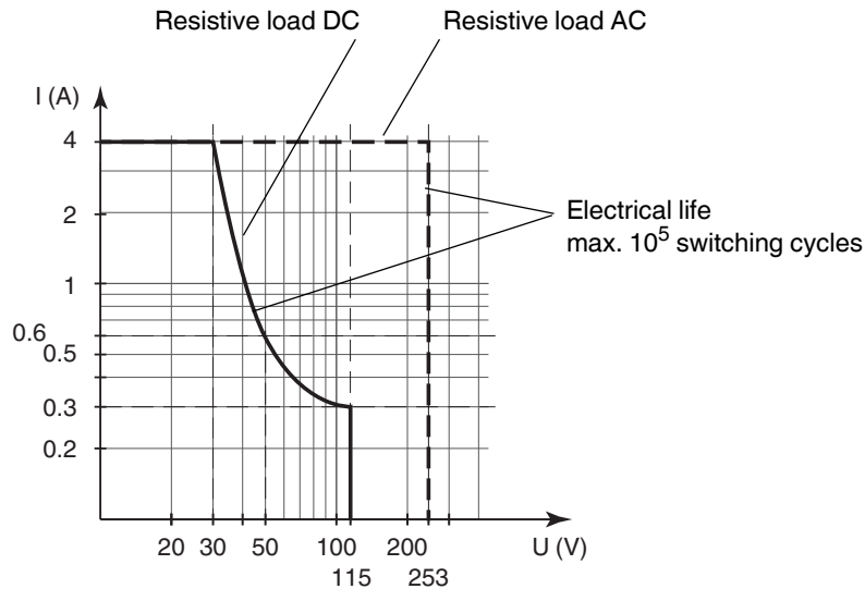
Maximum switching power of output contacts
